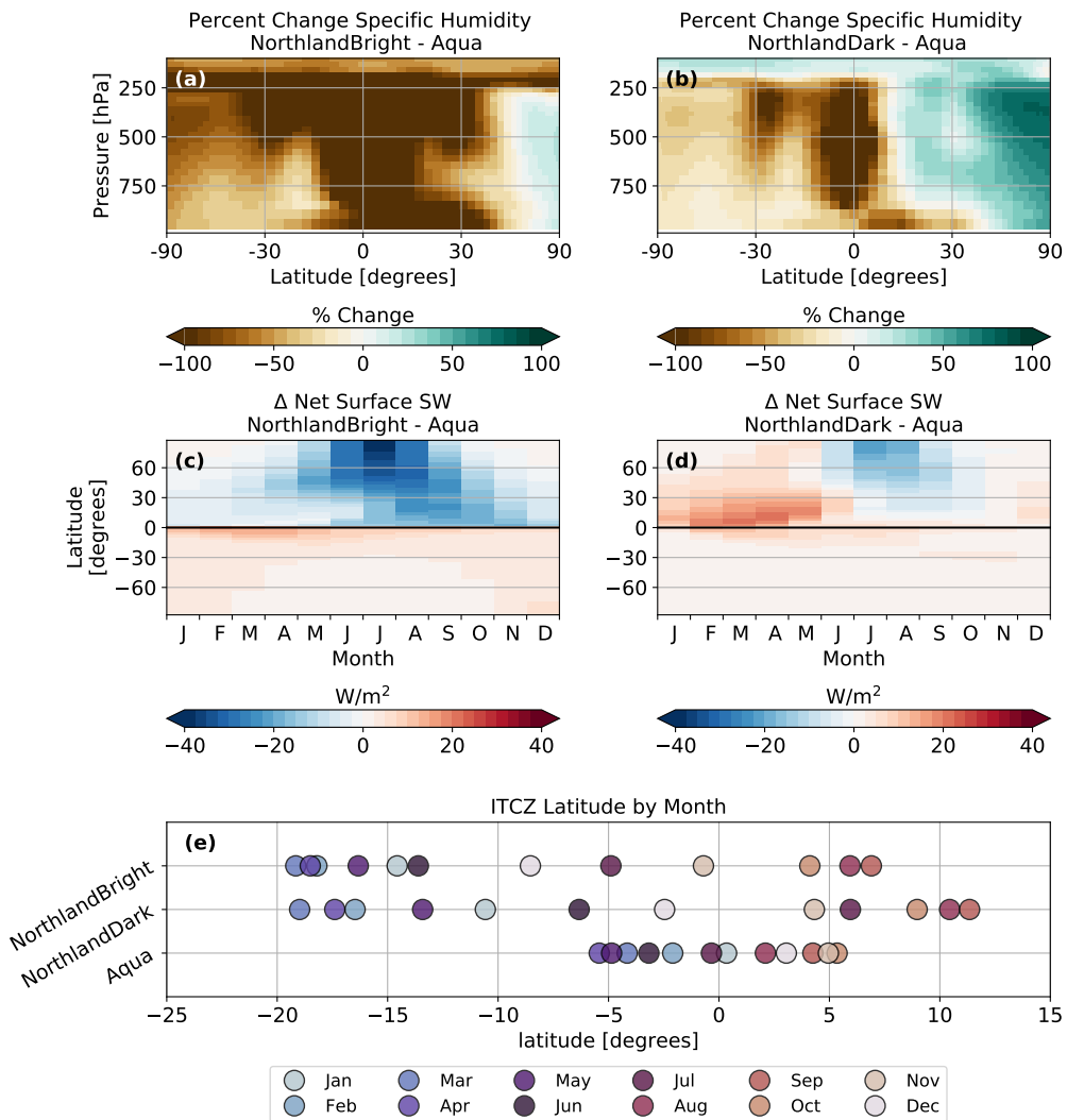
FIG. 10. Top: zonal mean percent change in annual mean specific humidity for (a) NorthlandBright - Aqua and (b) NorthlandDark - Aqua. Middle: seasonal cycle of the zonal mean change in net SW absorbed at the surface for (c) NorthlandBright - Aqua and (d) NorthlandDark - Aqua. Bottom: ITCZ latitude calculated as the center of mass of zonal mean precipitation from 30°S to 30°N for NorthlandBright, NorthlandDark, and Aqua, where each dot represents a single month of the year.
