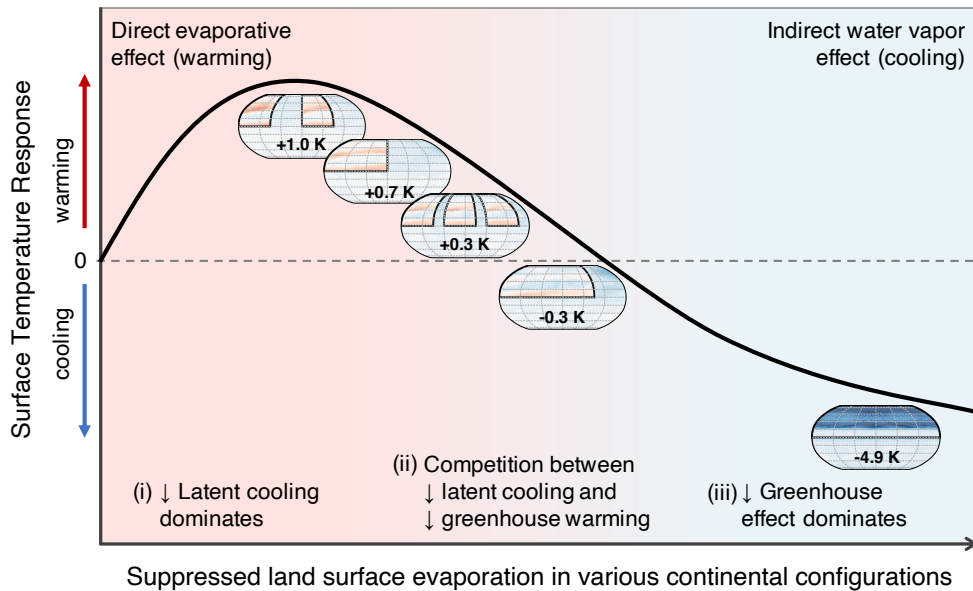
FIG. 13. Schematic showing the surface temperature response to suppressed terrestrial evaporation for a variety of NH continental configurations. Land area generally increases from left to right, though for a given total land area, larger continents sit farther to the right on the curve than smaller, more numerous continents. Qualitative locations of suppressing terrestrial evaporation on TwoPatchLand, NorthWestLand, ThreePatchLand, ThreeQuarterLand, and Northland are shown by the maps of temperature change for each continental configuration, with the annual mean change in land surface temperature noted on each map.
