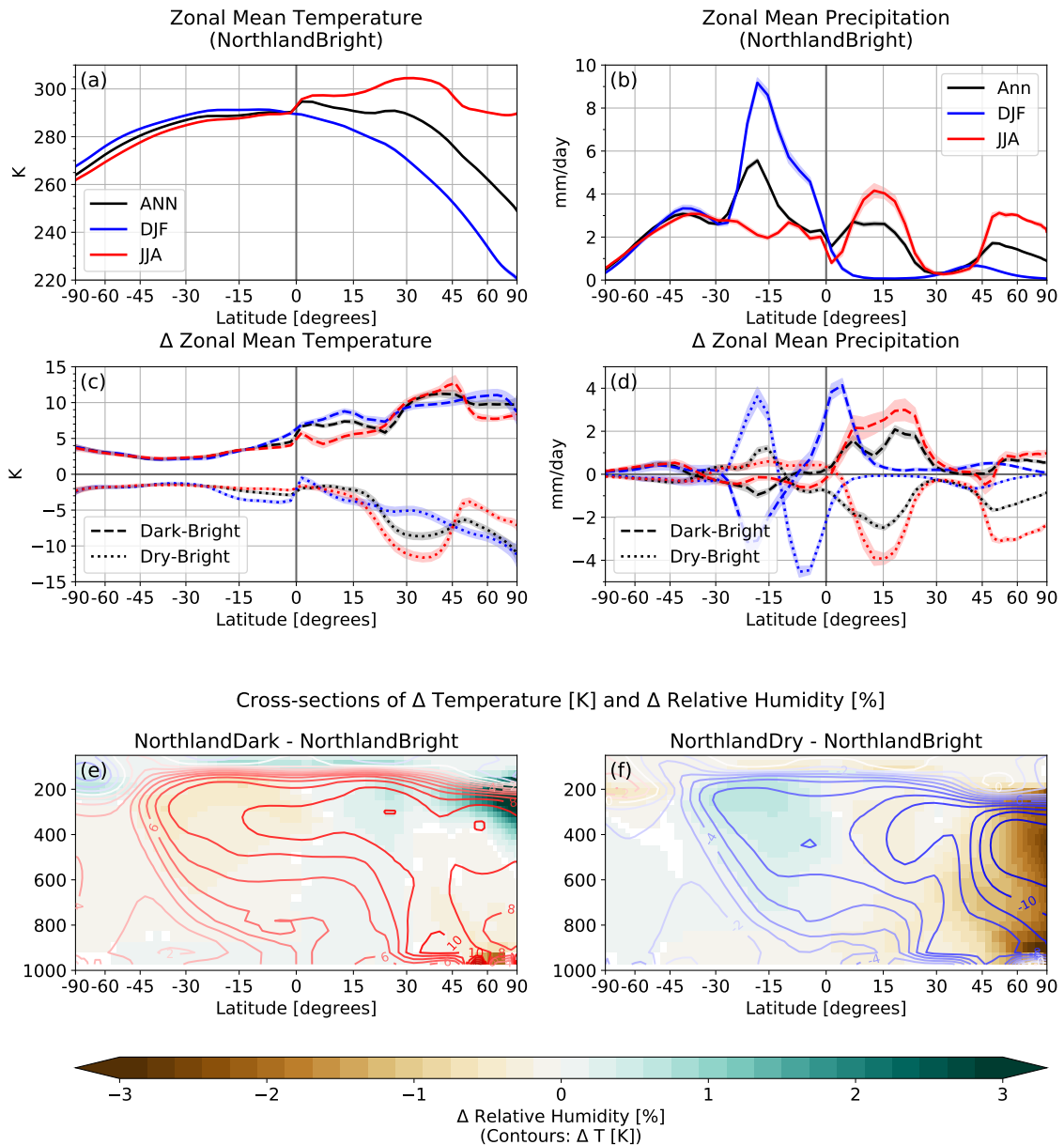
FIG. 2. Zonal mean temperature (a,c) and precipitation (b,d). The NorthlandBright simulation is shown in (a) & (b) (solid lines). The anomalies for NorthlandDark - NorthlandBright (dashed lines) and NorthlandDry - NorthlandBright (dotted lines) are shown in (c) & (d). In a-d, black lines indicate annual mean values, while blue (red) show values for December/January/February (June/July/August) in (a,c) and cyan (magenta) show values for February/March/April (August/September/October) in (b,d). Shading in a-d indicates \pm 1 standard deviation. Panels (e,f) show the annual mean change in zonal mean relative humidity (shading) and temperature (contours) for (e) NorthlandDark-NorthlandBright and (f) NorthlandDry-NorthlandBright. Temperature contours (red/blue lines in e-f) are spaced at 1K, with red values > 0 and blue values < 0 . Only humidity values in (e,f) which differ significantly ( p < 0.05 using a student's t-test) are shown.
