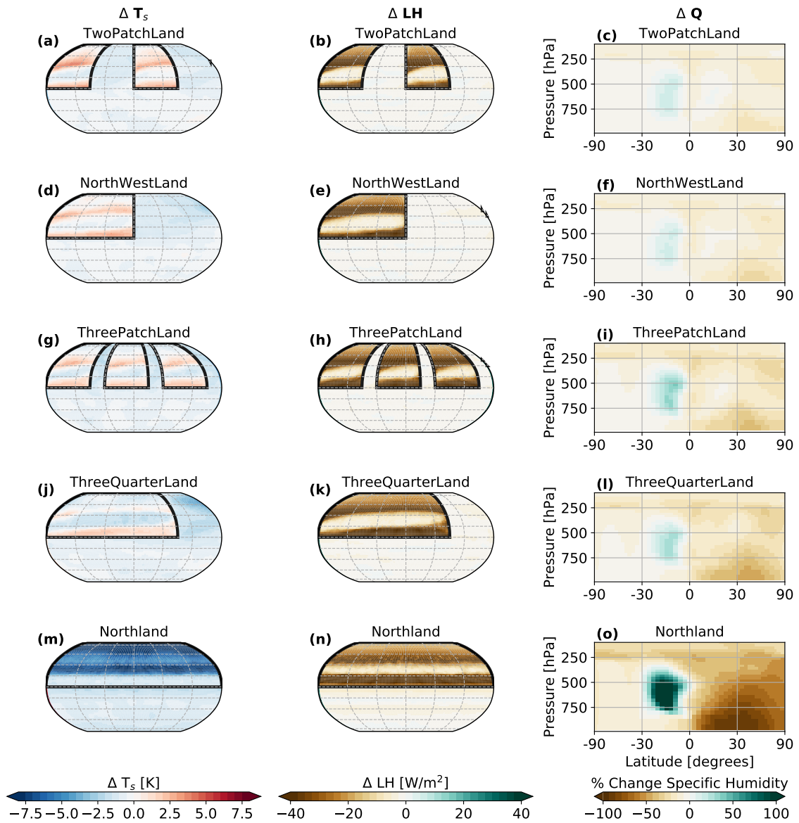
FIG. 7. Annual mean change in surface temperature (left), latent heat flux (center), and percent change in zonal mean specific humidity (right) for suppressing terrestrial evaporation in various continental configurations. Thick black lines show the continental boundary.
