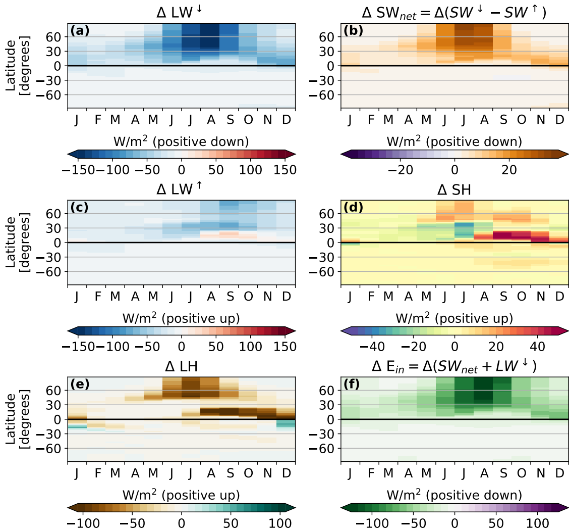
FIG. 5. Change in the zonal mean surface energy budget for NorthlandDry - NorthlandBright over the course of the year. The change in downwards LW is shown in (a) while the change in net SFC SW is shown in (b). LW emitted by the surface is shown in (c), while (d) and (e) show sensible and latent heat, respectively. (f) shows the change in net surface energy uptake ( E_{in} = SW^{\downarrow} - SW^{\uparrow} + LW^{\downarrow} ), where positive values indicate more energy into the surface; in the annual mean this would be balanced by E_{out} = LW^{\uparrow} + LH + SH .
