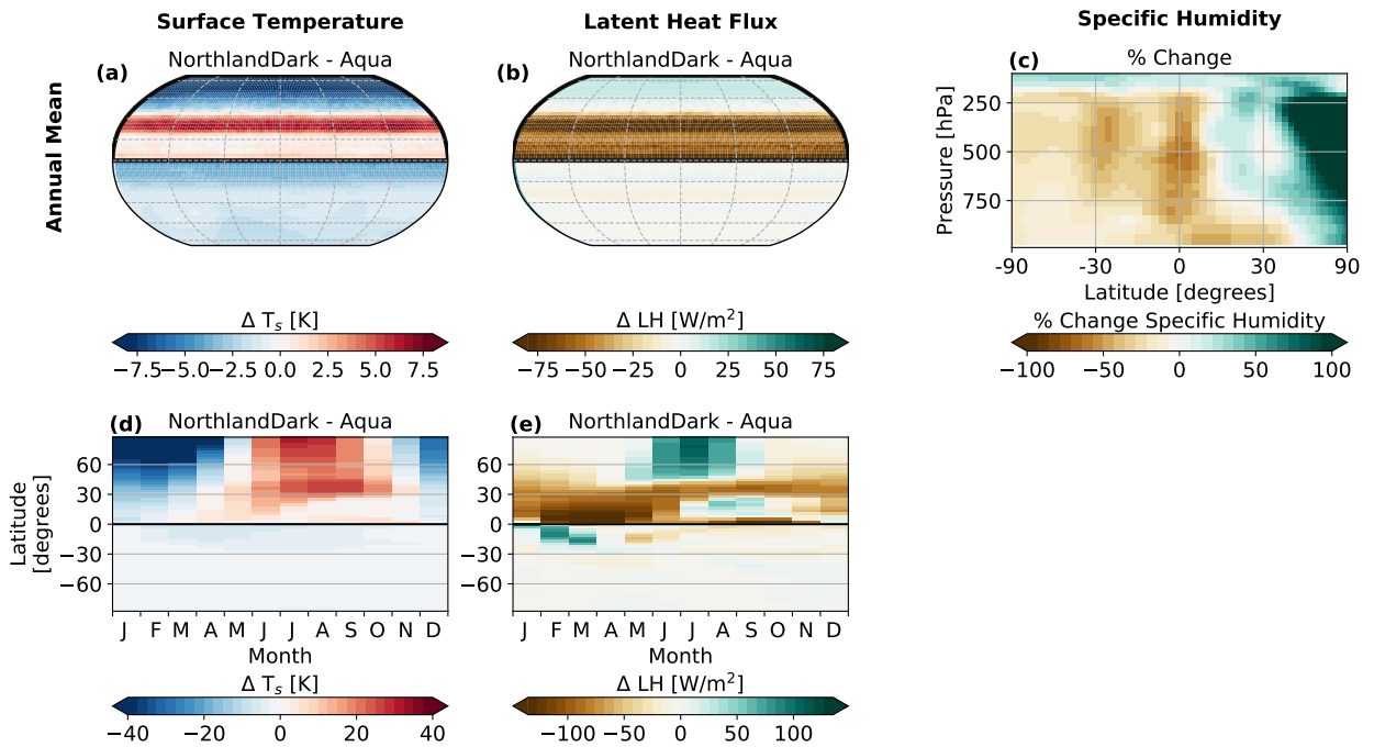
FIG. 9. Change in surface temperature (left), change in latent heat flux (center), and percent change in zonal mean specific humidity (right) between NorthlandDark and Aqua. The annual mean change is shown in a-c, while the zonal-mean seasonal cycle is shown in d-e.
