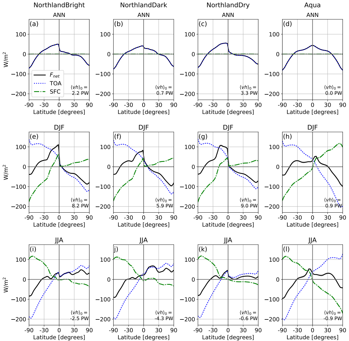
FIG. 12. Zonally averaged net TOA energy flux ( TOA , blue dotted line), net surface energy flux ( SFC , green dash-dot line), and the atmospheric column energy source ( F_{net} = TOA - SFC ; black solid line) for the annual mean (top row), DJF (middle row) and JJA (bottom row). NorthlandBright is shown in the first column, NorthlandDark in the second, NorthlandDry in the third, and Aqua in the fourth. The total column integrated cross-equatorial atmospheric energy transport (positive northwards) for each season is noted in the lower right of each panel.
